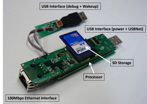
Figure 4: Photograph of the gumstix-based Somniloquy prototype - Wired-1NIC version.
