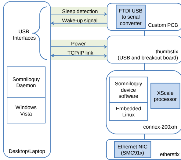
Figure 3: Block diagram of the Somniloquy prototype system - Wired-1NIC version. The figure shows various components of the gumstix and the USB interfaces to the host laptop.
